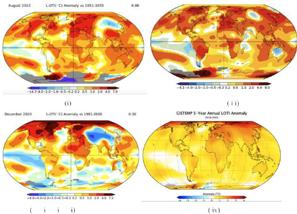
Figure 3a. Maps from another source: GISTEMP L-OTI (NASA) [35]; (i) 2022 (ref. 1951–1955); (ii) 2022 (ref. 1951–1980); (iii) 2020 (ref. 1981–2000); (iv) 2018–2022.
